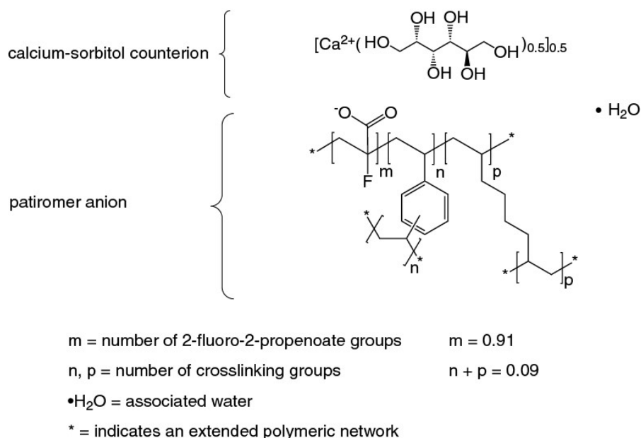
Figure 1: Chemical Structure of Patiomer Sorbitex Calcium
